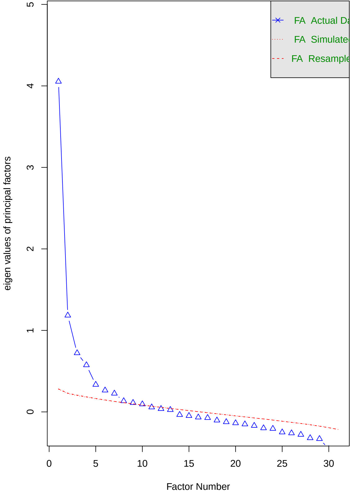
Parallel Analysis – Sweden
